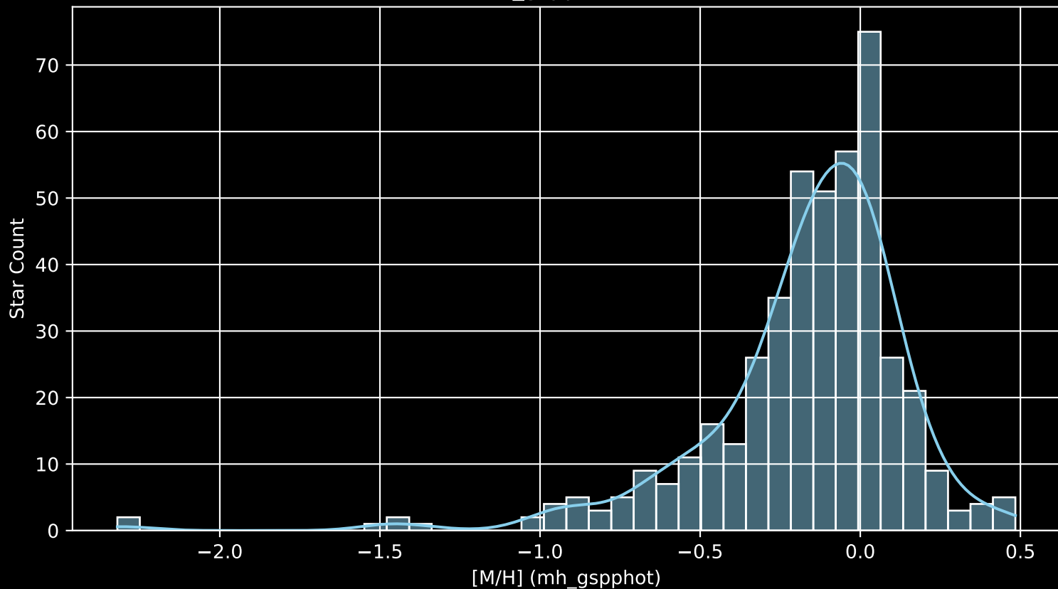
APOGEE DR17 Field: [195-04 [M/H] (mh_gspphot) (n= 447)
