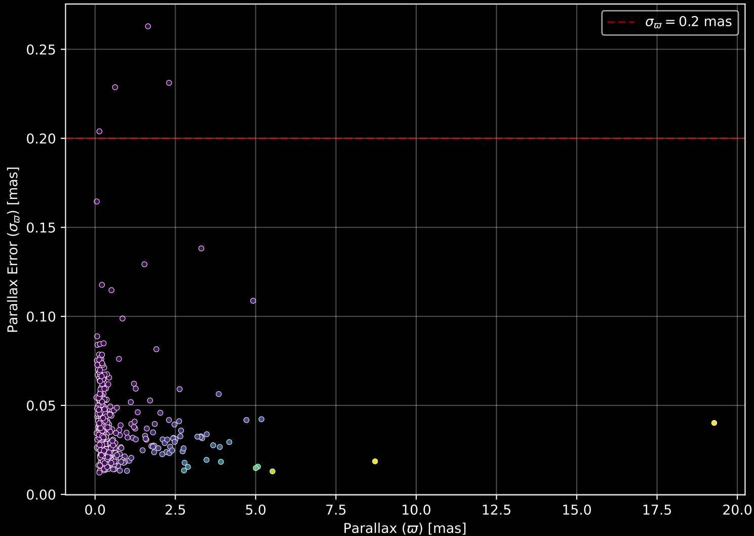
APOGEE DR17 Field: [195-04] Parallax Quality (n= 449)
