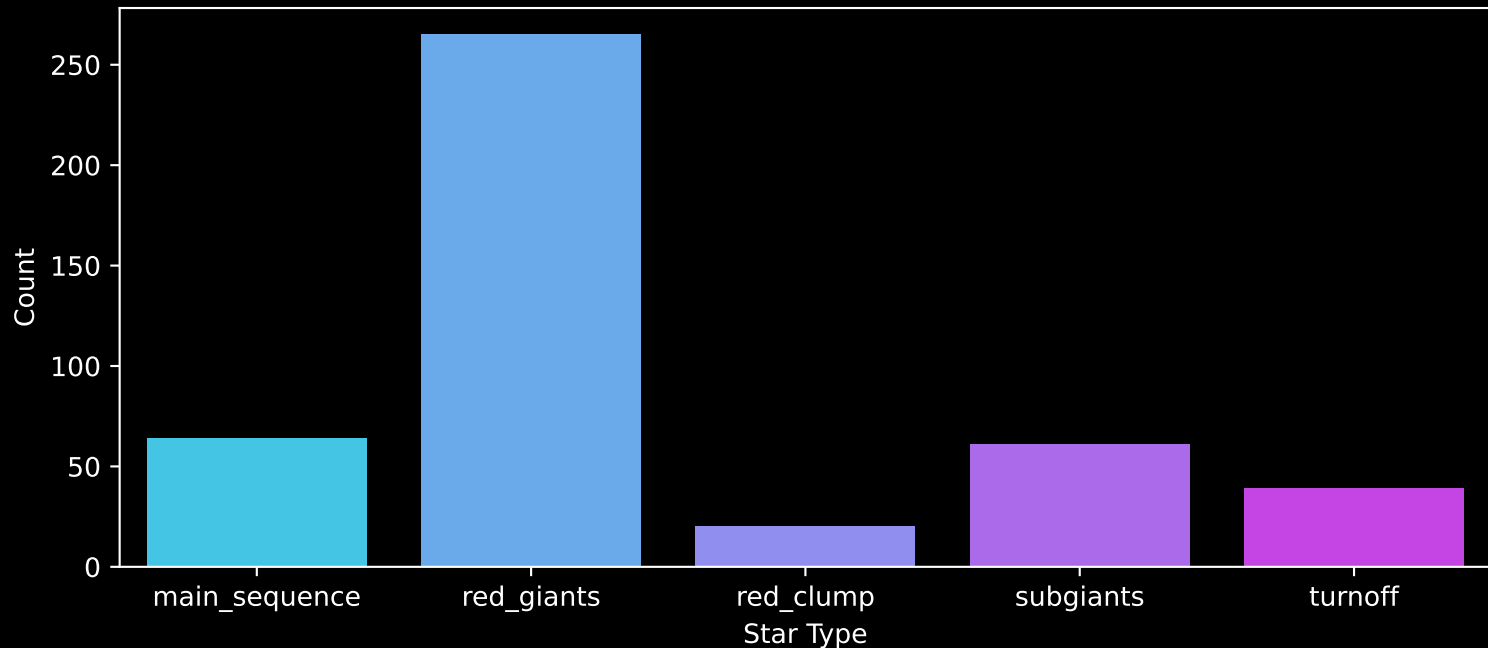
APOGEE DR17 Field: [195-04] Count plot of Star Type
