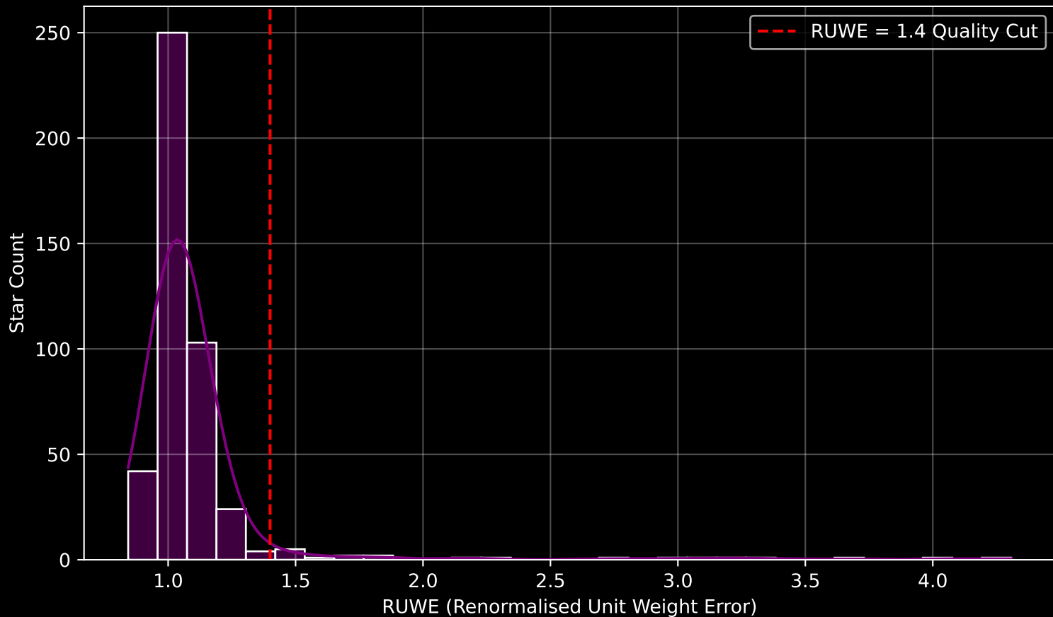
GAPOGEE DR17 Field [195-04] RUWE Distribution (n= 443)
