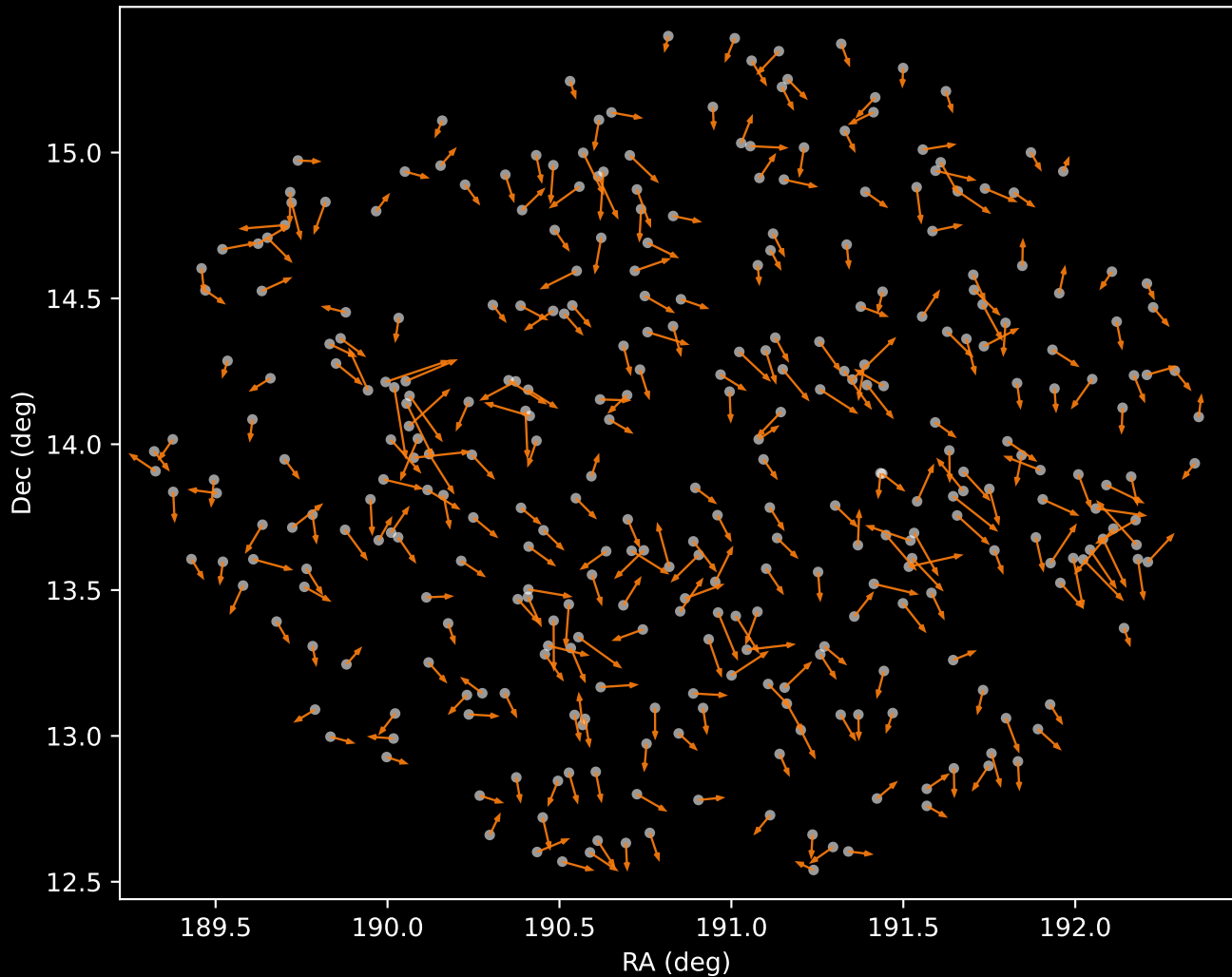
APOGEE DR17 Cluster 2 Proper Motion Vectors (n=327)
