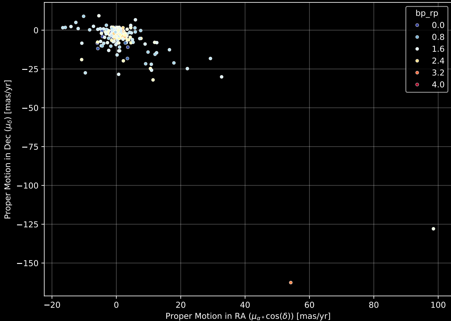
APOGEE DR17 Field: [195-04] Proper Motion Diagram (n= 449)
