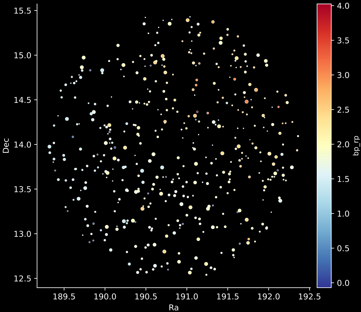
APOGEE DR17 Field: [195-04] Stars: 449
