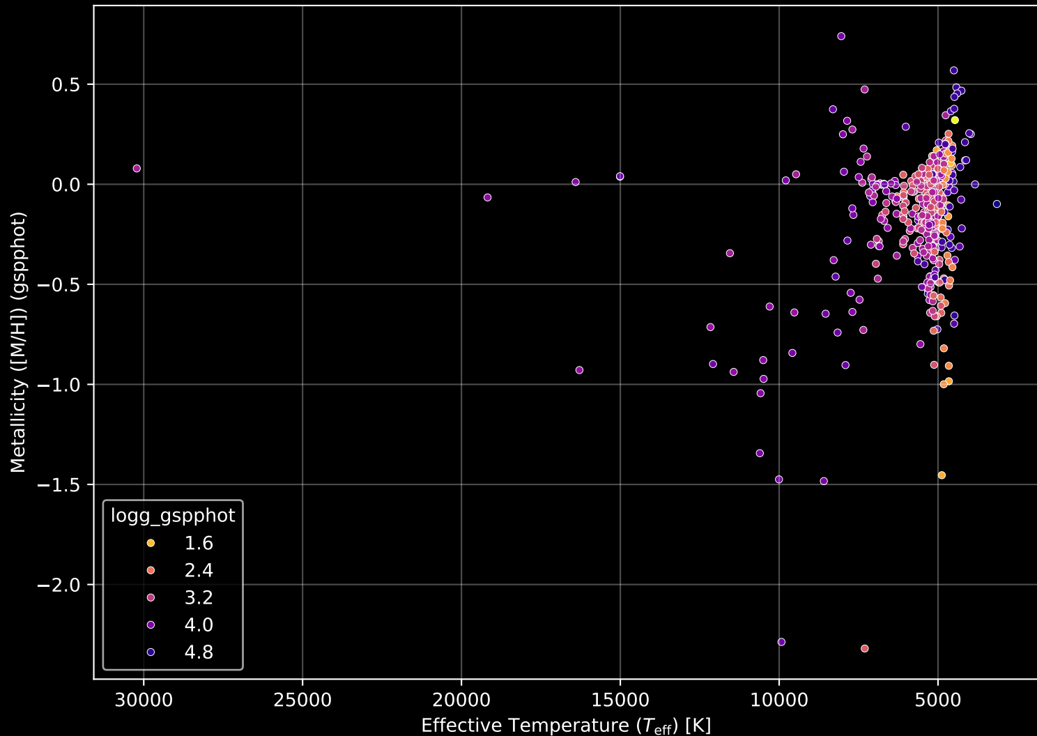
APOGEE DR17 Field: [195-04] Stellar Population Parameters (n= 449)
